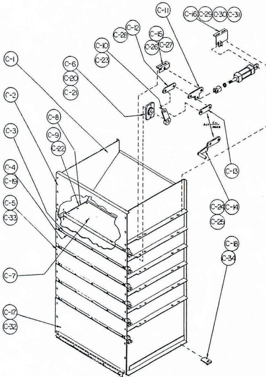
FIGURE NO. 3 COLLECTION CHUTES — GX-4, GX-5
